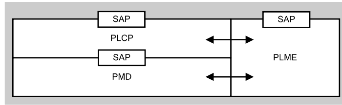
Figure 13.20 The PLCP and PMD sub-layers indicating the SAP interface with the abstract support from the PLME.
